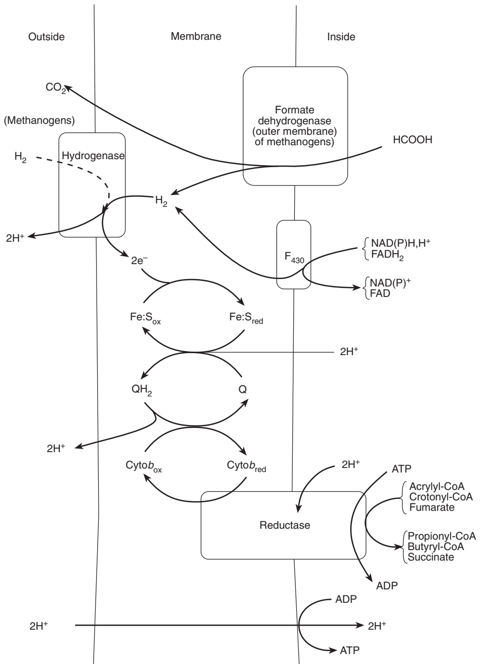
Fig. 6.4. Representation of anaerobic electron transport systems (putative). Not all components are found in all microorganisms nor are all components observed in ruminal microorganisms included. Based on Erfle et al. (1986).
