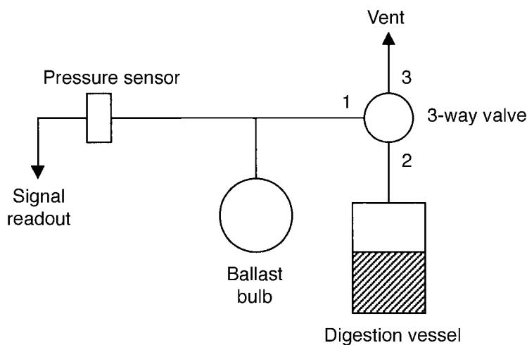
Fig. 10.1. Schematic view of a vented gas measurement system (redrawn from Beaubien et al. , 1988).
